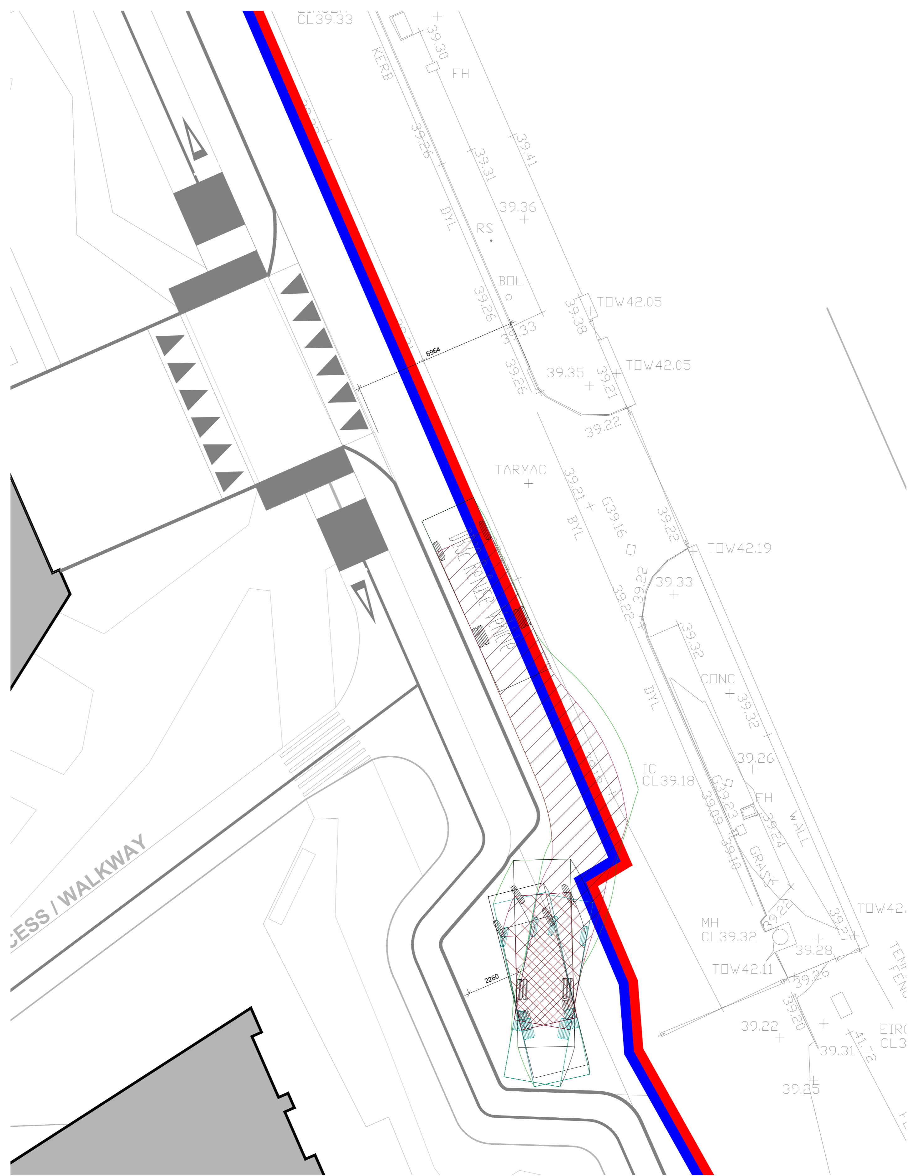
AUTOROUTE REFUSE VEHICLE TRACKING - REVERSE PARKING
