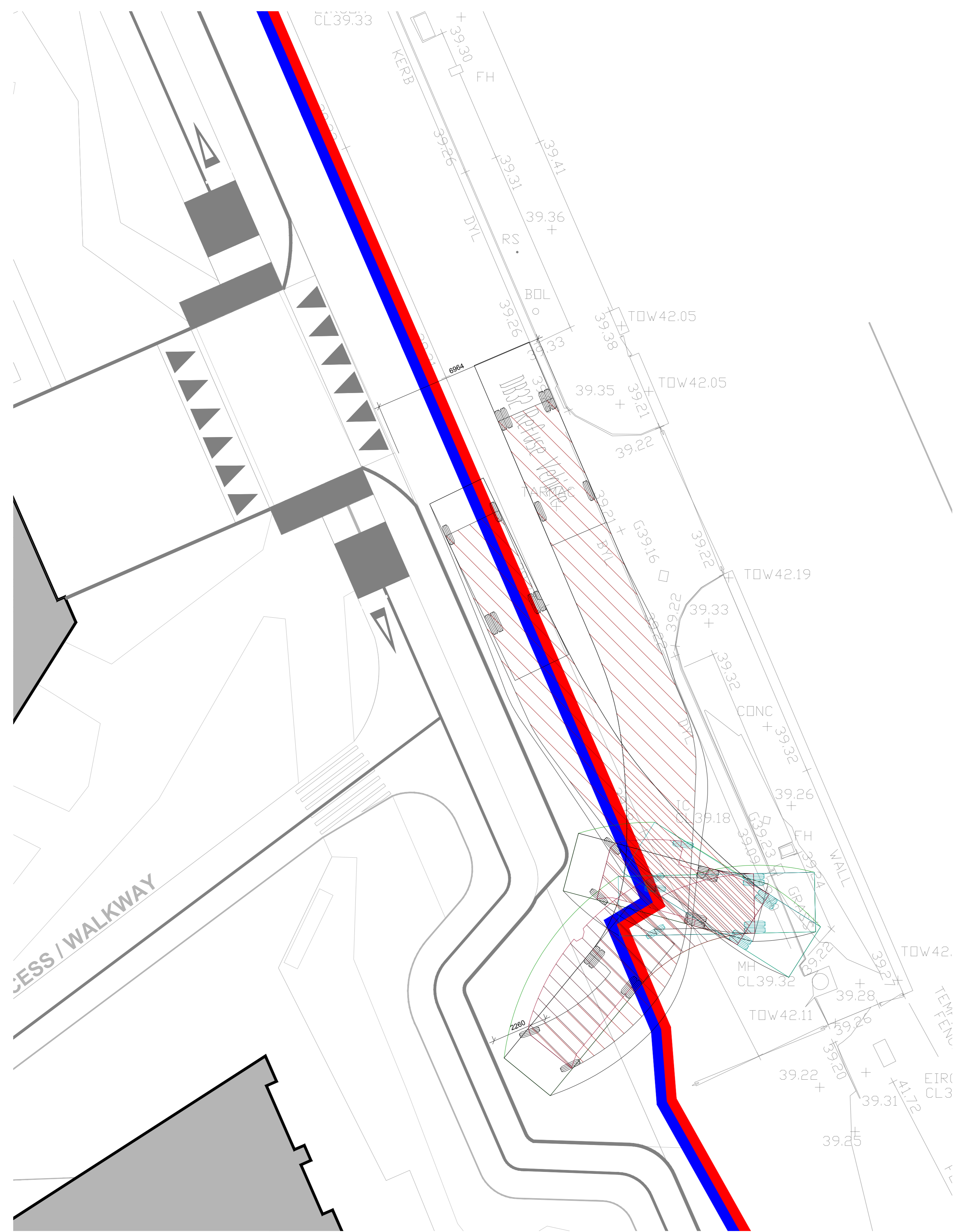
AUTOROUTE REFUSE VEHICLE TRACKING - TURNING
